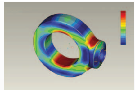
Typical rod end with loads applied in Creo Elements/Pro Mechanica.
